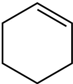
Cyclohexene
